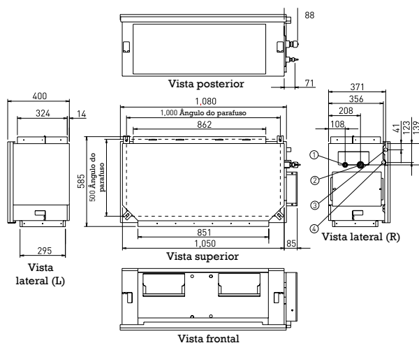
Modelo ACY125HUIAT-LH/ACY140HUIAT-LH
